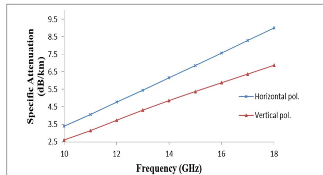
Fig. 3 Specific attenuation in Minna against frequency at 0.01% exceedance
