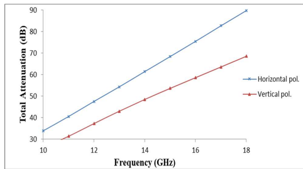
Fig. 4 Total attenuation in Minna against frequency at 0.01% exceedance
