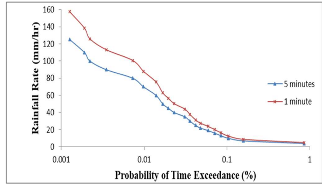
Fig. 2 Rainfall rate for Minna at percentage exceedance (0.001 – 1%)
