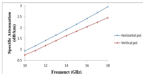
Fig. 6 Specific attenuation in Lapai against frequency at 0.01 % exceedance
