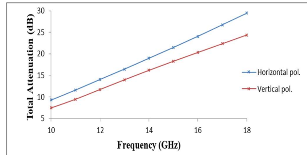
Fig. 7 Total attenuation in Lapai against frequency at 0.01 % exceedance
