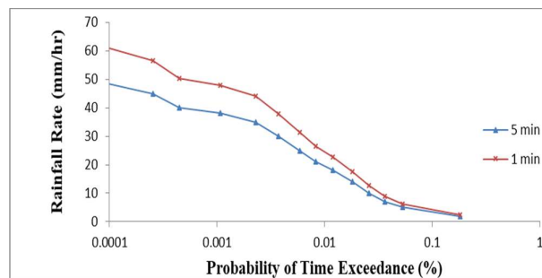
Fig. 5 Rainfall rate for Lapai at percentage exceedance (0.001 – 1%)
